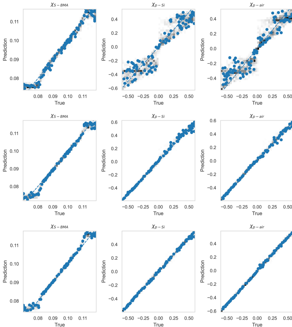
Fig. 10 Truth vs. prediction of the three \chi parameters for a hybrid model with an autoencoder and an MLP while varying the number of latent space parameters, n_1 = 2, 3 , and 4 in the top, middle, and bottom rows, respectively.
