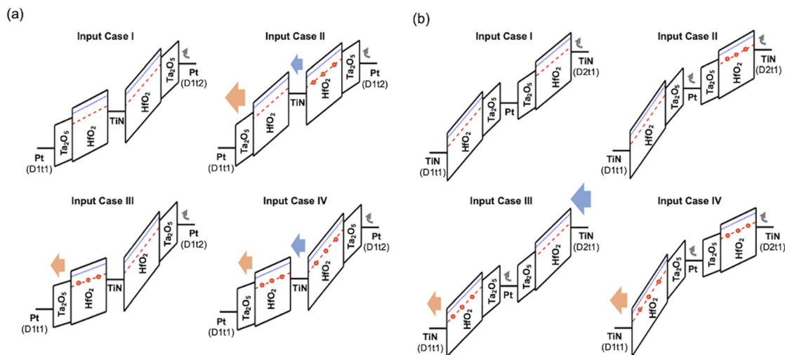
Fig. 7 Energy band diagram of AND and OR logic gates. (a) The ASM-two-2AND gate between D 1t1 and D 1t2 memristors and (b) ASM-two-2OR gate between D 1t1 and D 2t1 for each input case when a bias of +9 V and +12 V is applied for the logic operation, respectively.
