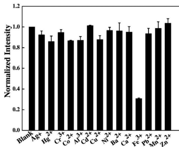
Fig. 9 Fluorescence response of the C-dots towards various metal ions (100 \mu M ). Adapted from Shen et al. , (2017) 146 with permission from Elsevier.
