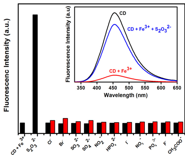
Fig. 8 Fluorescence changes in C-dots + Fe^{3+} in the presence of different anions. Adapted from Vandarkuzhali et al. , (2017) 139 with permission from Elsevier.
