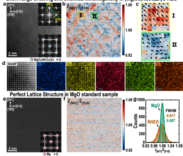
Fig. 2 HAADF-STEM image along the [100] zone axis for the rock-salt type (a) (Mg,Co,Ni,Cu,Zn)O HEO and (e) MgO standard sample with the corresponding FFT pattern in the top inset and the projected structure model at the bottom. (b and f) Lattice strain vectors overlaid on colormaps of the aspect ratios ( l_{[001]}/l_{[010]} ) for all quadrangle units in (a) and (e), respectively. (c) Enlargements of two types of domains in (b). (d) Atomic-resolution EDS elemental maps of Mg, Co, Ni, Cu, and Zn. (g) Comparison between the distributions of aspect ratios for (Mg,Co,Ni,Cu,Zn)O and MgO.
