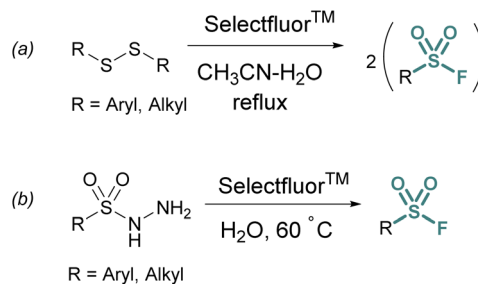
Fig. 3 Accessing sulfonyl fluorides with Selectfluor TM from (a) disulfides and (b) sulfonamides.
