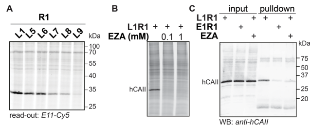
Fig. 7 (A) Labeling with R1-derived probes in HEK293 lysate. HEK293 cell lysate (2 mg \text{mL}^{-1} ) in HEPES (50 mM, pH 7.4) was incubated with R1-based iminoboronate probes (1 \mu\text{M} ) for 2 hours. Read-out with E11-Cy5 (1 \mu\text{M} ). (B) Labeling with L1R1 (10 \mu\text{M} ) in the presence of ethoxzolamide (EZA) (100 \mu\text{M} or 1 mM). Read-out with E11-Cy5 (10 \mu\text{M} ). (C) Western blot analysis of material retrieved from HEK lysate that was labeled with L1R1 or E1R1 (10 \mu\text{M} ) and subsequently subjected to an exchange reaction with E11-biotin. Input: aliquot taken before neutravidin enrichment of the labeled proteins; pulldown: material retrieved from the neutravidin beads. Read-out: immunoblot; primary antibody: rabbit polyclonal anti-human carbonic II; secondary antibody: donkey anti-rabbit 680.
