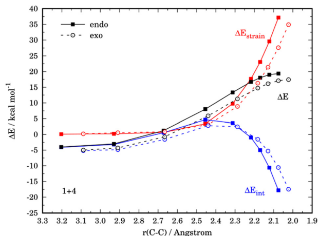
Fig. 8 Comparative activation strain analyses for the endo and exo pathways of the Diels–Alder cycloaddition reactions between the maleic anhydride ( 1 ) and 3-nitrofurán ( 4 ), projected onto the C...C bond-forming distance. All data have been computed at the M06-2X/def2-TZVPP level.
