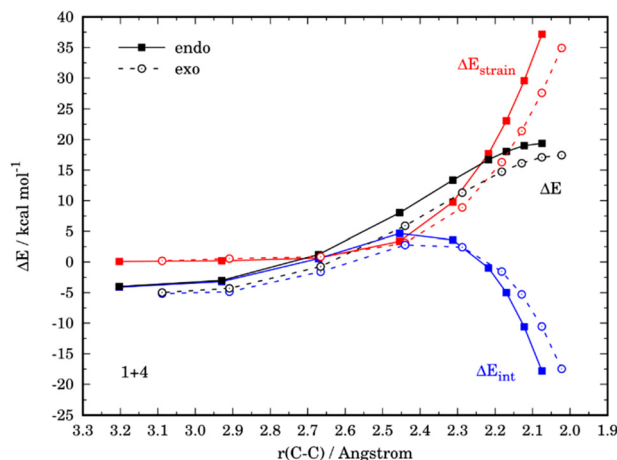
Fig. 8 Comparative activation strain analyses for the endo and exo pathways of the Diels–Alder cycloaddition reactions between the maleic anhydride ( 1 ) and 3-nitrofur ( 4 ), projected onto the C...C bond-forming distance. All data have been computed at the M06-2X/def2-TZVPP level.
