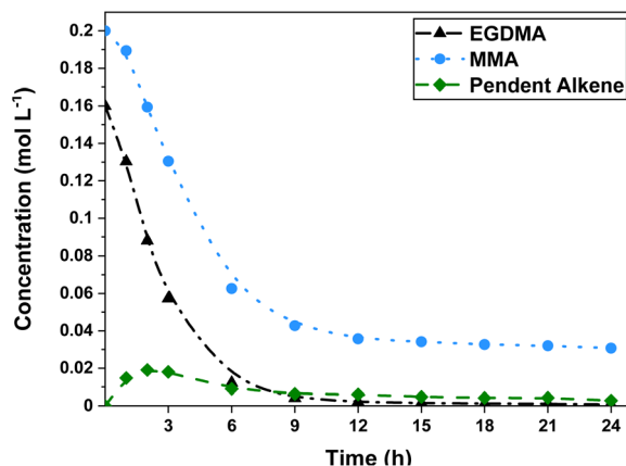
Fig. 3 Conversion of alkene protons observed by ^1\text{H} NMR spectroscopy. Experimental conditions: [\text{monomer}] : [\text{crosslinker}] : [\text{mRAFT agent}] : [\text{initiator}] of 10 : 8 : 1 : 0.3, 24 hours at 90 °C in toluene- d_8 .
