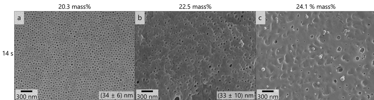
Fig. 5 Topography images by SEM of the membrane surfaces cast from solutions of PSAN 83 - b -PHEMA 17 82 in THF/DMF/DOX 3:1:1 using the 100 \mu m blade gap at 20.3 mass% (a), 22.5 mass% (b) and 24.1 mass% (c) with an evaporation time of 14 s.
