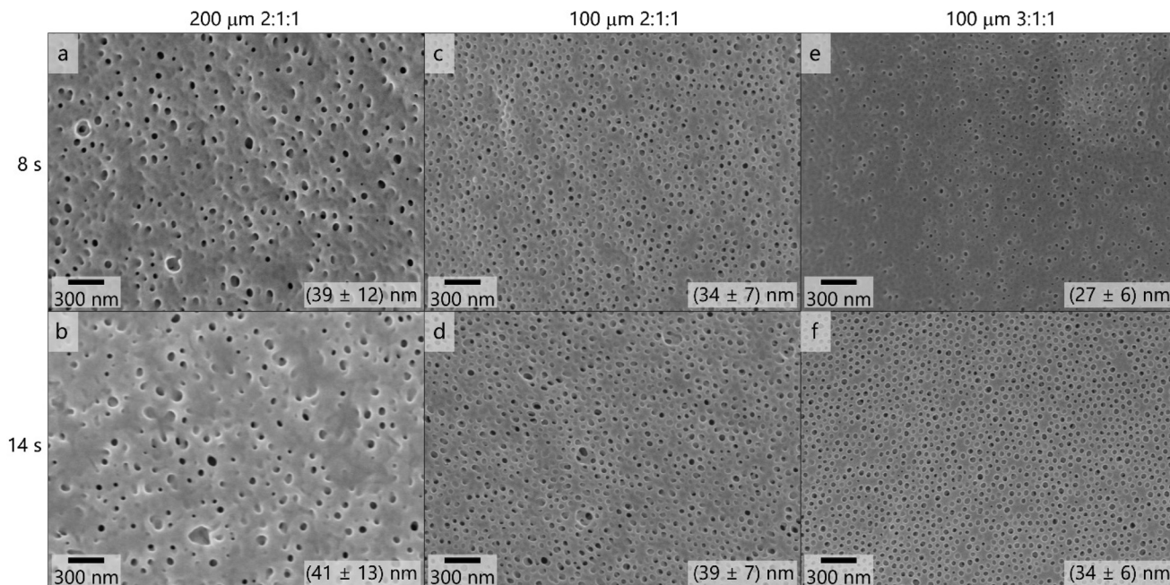
Fig. 4 Topography images by SEM of the membrane surfaces cast from solutions of PSAN 83 - b -PHEMA 17 82 in THF/DMF/DOX 2:1:1 (a–d) and 3:1:1 (e and f) at 20.3–20.5 mass% using 200 \mu m (a and b) and 100 \mu m (c–f) blade gap with varying evaporation times of 8 s (a, c and e) and 14 s (b, d and f), respectively. At the bottom right of each image the pore diameters measured visually (ImageJ) at more than 100 pores are displayed.
