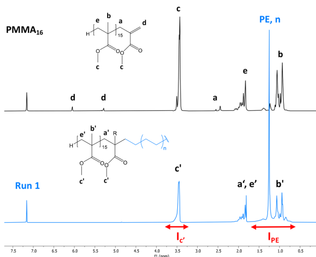
Fig. 2 ^1\text{H} NMR spectra (TCE/ \text{C}_6\text{D}_6 at 90 \text{ }^\circ\text{C} ) of the dry extract (a) from the \text{PMMA}_{16} seed latex and (b) from the latex obtained by ethylene emulsion polymerization in the presence of \text{PMMA}_{16} (run 1, Table 2).
