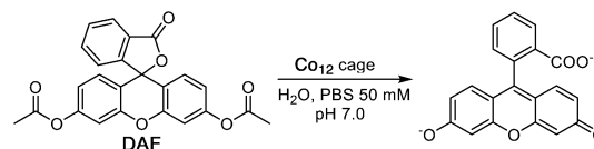
Scheme 2 Hydrolysis of diacetyl fluorescein.
