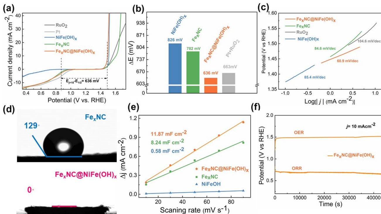
Fig. 3 (a) The polarization curves of different electrodes. (b) Potential difference ( \Delta E ) of \text{NiFe}(\text{OH})_x , \text{Fe}_x\text{NC} , \text{Fe}_x\text{NC@NiFe}(\text{OH})_x , and \text{Pt} + \text{RuO}_2 . (c) OER Tafel slopes. (d) Contact angle evaluation on \text{Fe}_x\text{NC} and \text{Fe}_x\text{NC@NiFe}(\text{OH})_x . (e) ECSA results of different electrodes. (f) The voltage-time curves of \text{Fe}_x\text{NC@NiFe}(\text{OH})_x at 10 \text{ mA cm}^{-2} .
