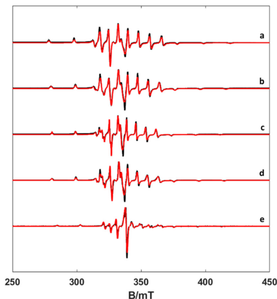
Fig. 2 X-band CW EPR spectra of frozen solutions of complexes (a) [VO(H 2 O) 5 ] 2+ , (b) [VO(nta)(H 2 O)] - , (c) [VO(Hdtppa)] 2- , (d) [VO(ox) 2 (H 2 O)] 2- , and (e) [VO(acac) 2 (H 2 O)] (experimental black line, simulation red one) at 77 K, 1 mW power and 0.2 mT modulation amplitude.
