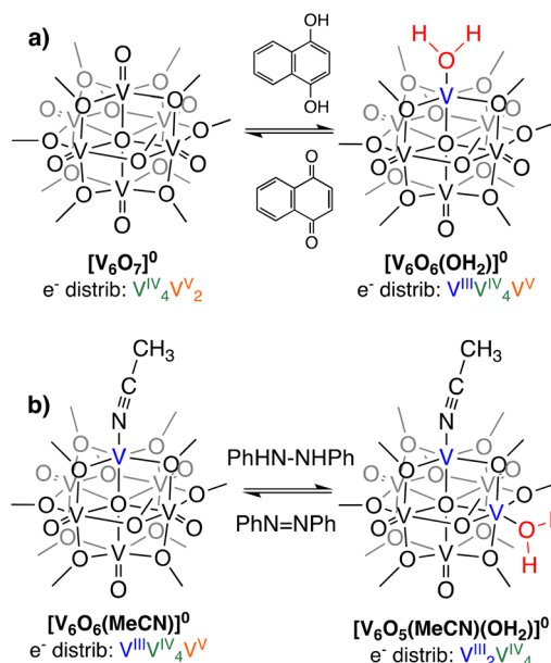
Scheme 2 Equilibrium reactions employed in the determination of BDFE(O–H) avg for (a) [\text{V}_6\text{O}_6(\text{OH}_2)]^0 and (b) [\text{V}_6\text{O}_5(\text{MeCN})(\text{OH}_2)]^0 .
