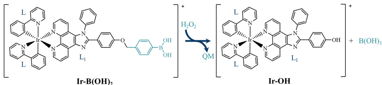
Scheme 1 Structures of complexes Ir-B(OH) 2 and Ir-OH .
