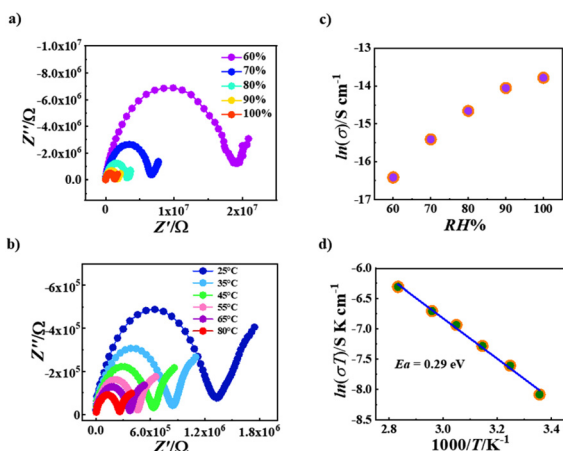
Fig. 6 Nyquist plots for R-1 at 25 °C under different relative humidity (RH) levels (a). Nyquist plots for R-1 at different temperatures under 100% relative humidity (RH) (b). Plots of proton conductivity vs. RH for R-1 at 25 °C (c). Plots of \ln(\sigma T) vs. 1000/T for R-1 under 100% relative humidity (RH) (d).
