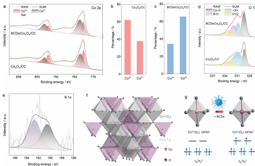
Fig. 2 Surface property characterization. (a) XPS spectra of the Co 2p region of the \text{Co}_3\text{O}_4/\text{CC} and \text{BCDs}/\text{Co}_3\text{O}_4/\text{CC} . (b and c) Calculated ratio of \text{Co}^{3+} and \text{Co}^{2+} in \text{Co}_3\text{O}_4/\text{CC} and \text{BCDs}/\text{Co}_3\text{O}_4/\text{CC} , respectively. (d) O 1s region of \text{Co}_3\text{O}_4/\text{CC} and \text{BCDs}/\text{Co}_3\text{O}_4/\text{CC} . (e) B 1s region of \text{BCDs}/\text{Co}_3\text{O}_4/\text{CC} . (f) Crystal structure of \text{Co}_3\text{O}_4 . (g) Scheme of the valence electron configurations and spin states of octahedral Co influenced by the BCDs.
