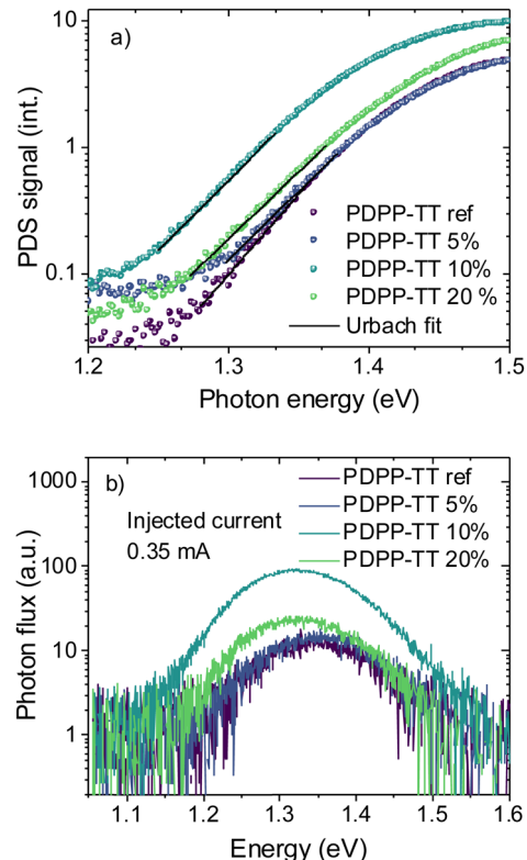
Fig. 4 (a) Photothermal deflection spectroscopy (PDS) spectra of polymer-PC71BM BHJ blend films, (b) electroluminescence (EL) spectra (uncorrected for detector sensitivity) measured at the same exposure time, of OSCs based on BHJ blends having various PDPP-TT polymer analogs with varying amounts of encapsulated units in the polymer backbone.
