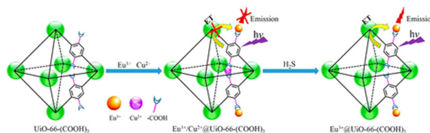
Fig. 6 Post-synthetic incorporation of \text{Eu}^{3+} and \text{Cu}^{2+} in \text{UiO-66}(\text{COOH})_2 to form \text{Eu}^{3+}/\text{Cu}^{2+}@\text{UiO-66}(\text{COOH})_2 , followed by the detection of \text{H}_2\text{S} . Reproduced with permission from ref. 84, the American Chemical Society, Copyright 2016.
