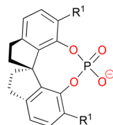
(R)-90 (R 1 = 2,4,6- i -Pr 3 -C 6 H 2 )
