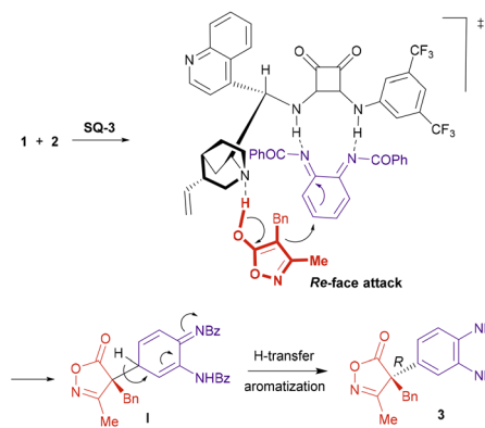
Scheme 6 Mechanistic and stereochemical proposal for the arylation reaction.
