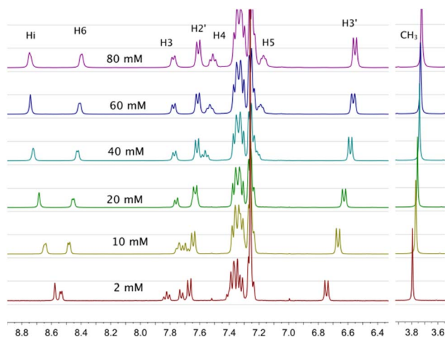
Fig. 5 ^1\text{H} -NMR spectra of [\text{Cu}(\text{NN}'\text{-OCH}_3)(\text{PPh}_3)\text{Br}] , T = 220\text{ K} , for several concentrations used to calculate self-association constants. Proton assignment is included. Similar behaviors were observed at different temperatures (see Tables SI3a to g†).
