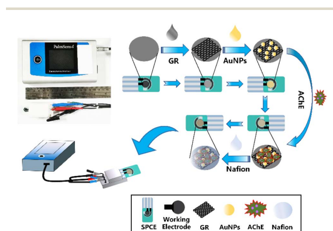
Fig. 1 Preparation process of SPCE/GR/AuNPs/AChE/Nafion.
