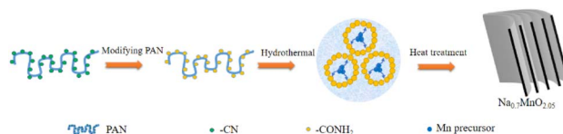
Fig. 1 Schematic synthesis process of hierarchical book-like \text{P2-Na}_{0.7}\text{MnO}_{2.05} .
