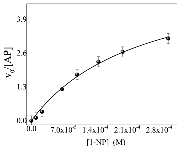
Fig. 2 Effect of 1-NP concentration on the initial reaction rate ( v_0 ) of 1-NP hydrolysis catalyzed by AP at \text{pH} = 10 , T = 35^\circ\text{C} , [\text{AP}] = 1.0 \times 10^{-7}\text{ M} . [1\text{-NP}] : 1.0 \times 10^{-5}\text{ M} , 2.3 \times 10^{-5}\text{ M} , 6.7 \times 10^{-5}\text{ M} , 1.0 \times 10^{-4}\text{ M} , 1.5 \times 10^{-4}\text{ M} , 2.0 \times 10^{-4}\text{ M} , 3.0 \times 10^{-4}\text{ M} . The experimental data were fitted according to the eqn (1), (—) solid lines.
