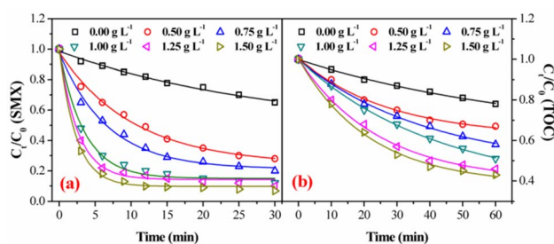
Fig. 6 Effect of catalyst dosage on degradation (a) and mineralization (b) of SMX in FeSO/O 3 (experiment conditions: [SMX] 0 = 20 mg L -1 , ozone dosage = 0.4 mg min -1 , initial pH = 7.0, T = 20 ± 1 °C).
