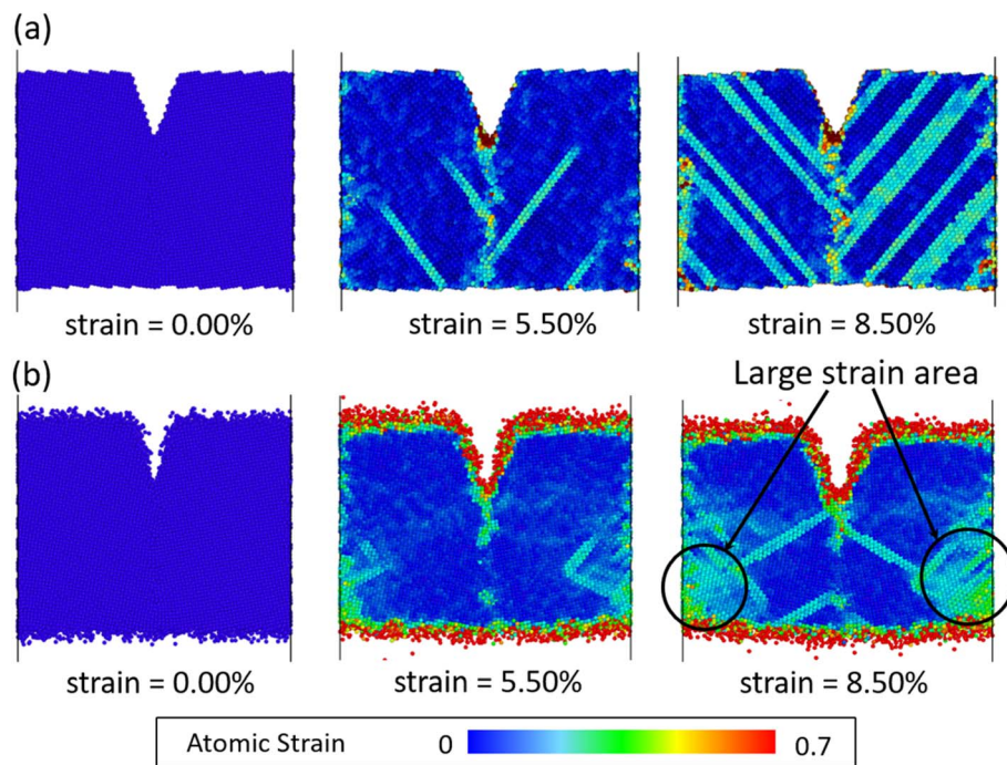
Fig. 3 Atomic shear strain of \text{Fe}_{40}\text{Ni}_{40}\text{Cr}_{20} alloy in (a) vacuum and (b) high-temperature/pressure water environments. Non-reacted water molecules in (b) are invisible for clarity.
