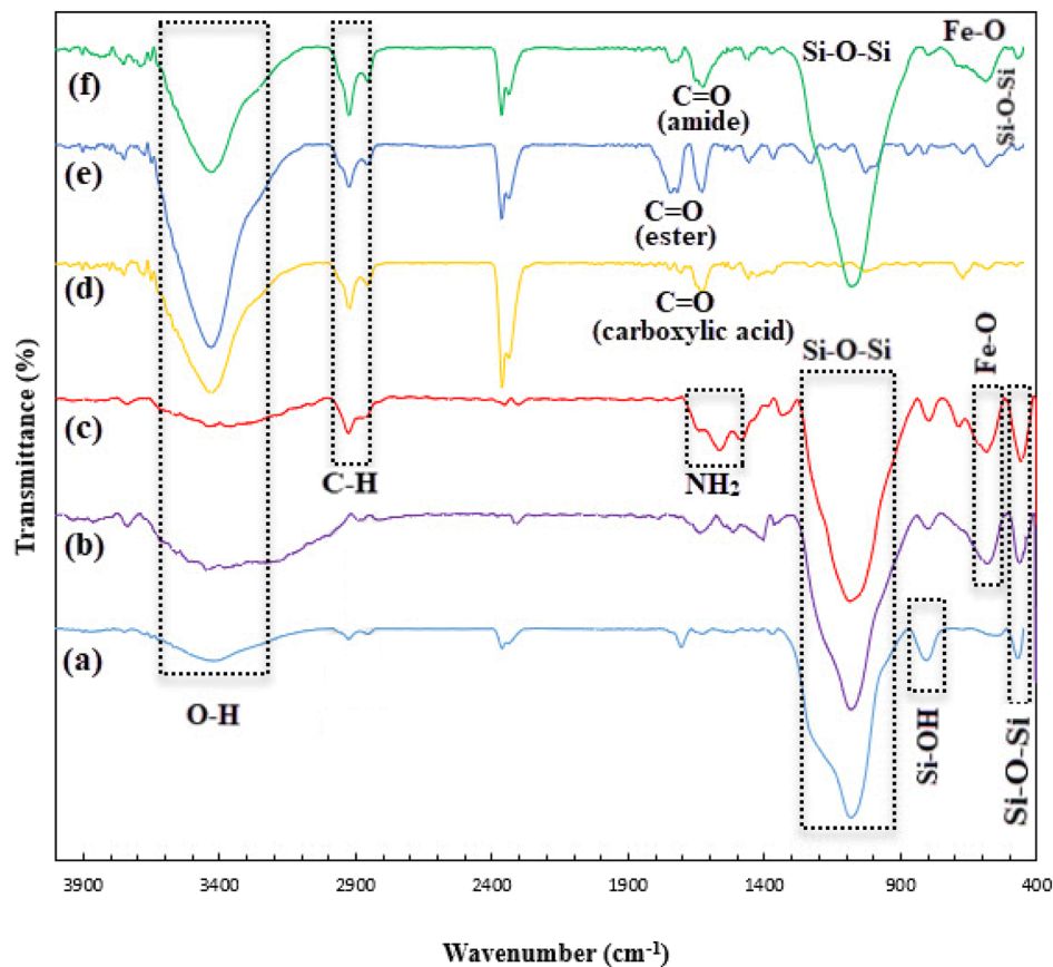
Fig. 2 FTIR spectra of (a) SBA-15, (b) SBA-15/ \text{Fe}_3\text{O}_4 , (c) SBA-15/ \text{Fe}_3\text{O}_4 - \text{NH}_2 , (d) alginic acid, (e) methyl-esterified alginic acid, and (f) Alg@SBA-15/ \text{Fe}_3\text{O}_4 .
