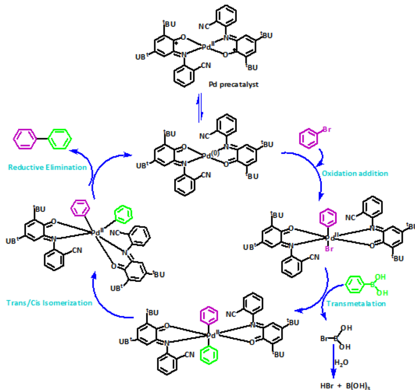
Scheme 5 The suggested mechanism for Suzuki reaction with Pd II L 2 NIS
