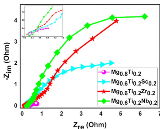
Fig. 9 Nyquist plots of \text{Mg}_{0.8}\text{Ti}_{0.2} , \text{Mg}_{0.6}\text{Ti}_{0.2}\text{Sc}_{0.2} , \text{Mg}_{0.6}\text{Ti}_{0.2}\text{Zr}_{0.2} and \text{Mg}_{0.6}\text{Ti}_{0.2}\text{Nb}_{0.2} alloys.
