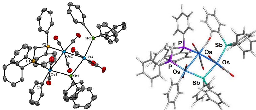
Fig. 4 Molecular structure (left, 4 ) and M06-optimized structure (right, species D ) of [\text{Os}_3(\text{CO})_8(\text{SbPh}_3)(\eta^1\text{-Ph})(\mu\text{-SbPh}_2)(\mu\text{-dppm})] showing 50% probability atomic displacement ellipsoids. Hydrogen atoms are omitted for clarity.
