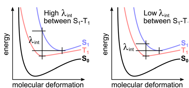
Fig. 1 Jablonski diagrams of a molecular system with high (left) and low (right) reorganization energy with ground state S_0 (black), excited singlet state S_1 (blue) and excited triplet state T_1 (red).
