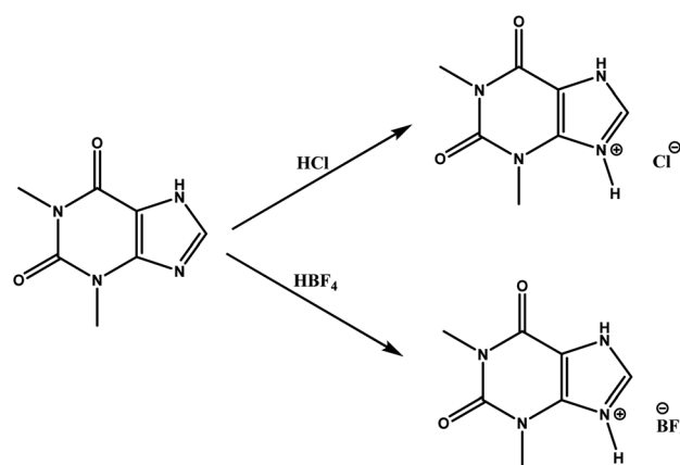
Fig. 2 General scheme of additives synthesis.
