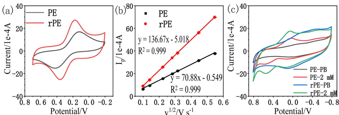
Fig. 2 (a) CVs of the paper electrodes in 1 mM \text{K}_3\text{Fe}(\text{CN})_6 in 1 M KCl. Scan rate = 50 mV s -1 . (b) Plots of oxidation peak current ( I_p/10^{-4} A) vs. square root of the scan rate ( \nu^{1/2} ) for PE and rPE. (c) CVs of PB (pH 7) and 2 mM amitrole. Scan rate = 50 mV s -1 .
