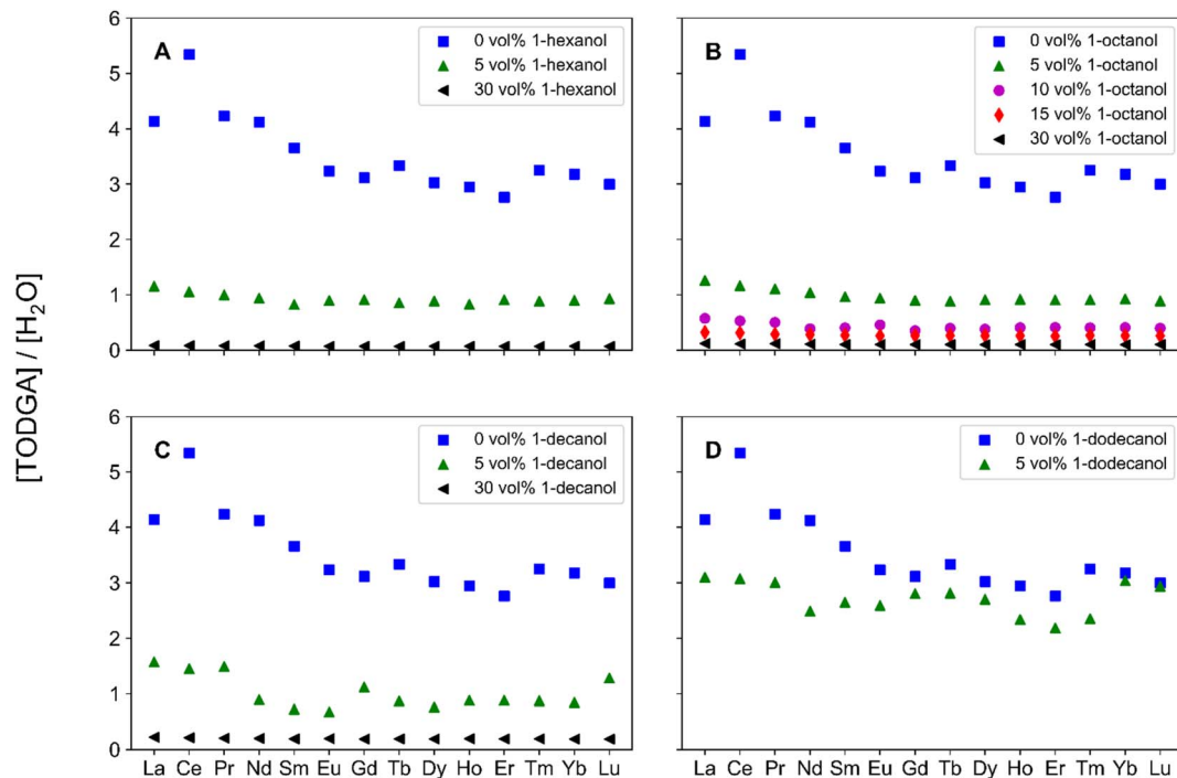
Fig. 3 Calculated unbound TODGA per extracted H 2 O molecule, across the Ln period for organic phases containing (A) 0 vol%, 5 vol%, or 30 vol% 1-hexanol, (B) 0 vol%, 5 vol%, 10 vol%, 15 vol%, or 30 vol% 1-octanol, (C) 0 vol%, 5 vol%, or 30 vol% 1-decanol, and (D) 0 vol% or 5 vol% 1-dodecanol. For each system tested, 0 vol% (blue, squares), 5 vol% (green triangles), 10 vol% (magenta circles), 15 vol% (red diamonds), and 30 vol% (black left-triangles).
