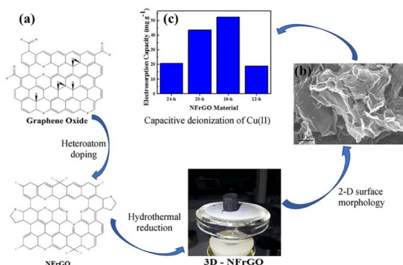
Fig. 19 (a) Illustration of fabrication of 3-dimensional N, F-codoped reduced graphene oxide (NFrGO); (b) SEM image of NFrGO fabricated at 16 h; (c) copper electrosorption capacity of NFrGO electrode materials after 120 min of incubation in CDI system. (Reproduced with permission from ref. 112 Copyright 2021 Elsevier.)
