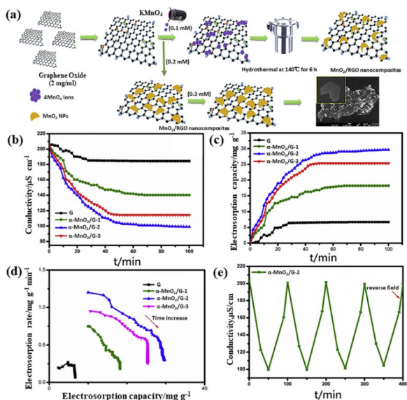
Fig. 8 (a) Illustration of the nucleation growth mechanism of MnO 2 /G nanocomposites; (b) plots of conductivity vs. time; (c) electroadsorption capacity vs. time; (d) CDI Kim-Yoon plots for G, α-MnO 2 /G-1, α-MnO 2 /G-2, and α-MnO 2 /G-3 electrodes; (e) desalination-regeneration profile of the α-MnO 2 /G-2 in a 100 mg per L NaCl at 1.2 V with a flow rate of 10 mL min -1 . (Reproduced with permission from ref. 76 Copyright 2020 Elsevier.)
