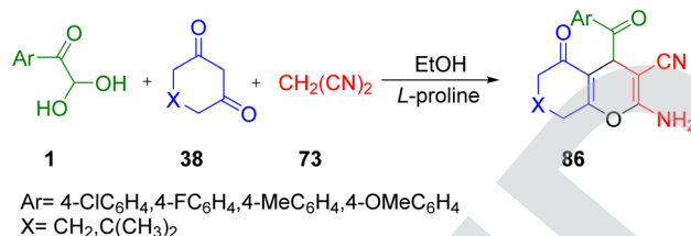
Scheme 55 Formation of 2-amino-4-aroxy-5-oxo-5,6,7,8-tetrahydro-4 H -chromene-3-carbonitrile 86 . 79
