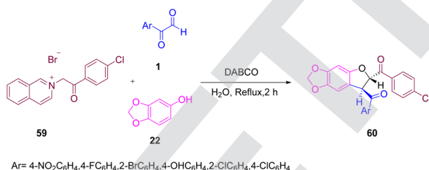
Scheme 30 Synthesis of trans -(4-chloroAryl)-7-aryl-6,7-dihydro(1,3)dioxolo(4,5- f )(1)benzofuran-6-yl)methanones 60 in a one-pot approach using DABCO. 61
