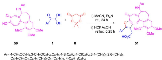
Scheme 23 Synthesis of 6,7-dihydrobenzo[9,10] heptaleno[3,2- b ]furan-9(5 H )-one 51 using Meldrum's acid 8 and colchicine 50 . 56
