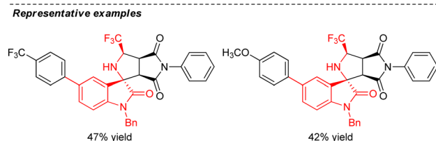
Scheme 6 Phase transfer-catalyzed stereoselective formation of spiro-fused [succinimide-pyrrolidine-oxindoles].
