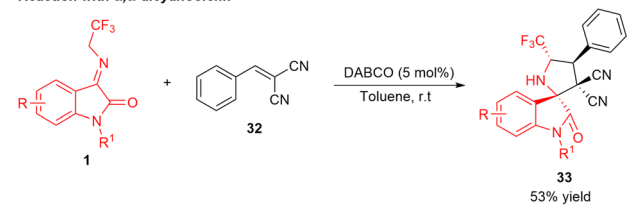
Scheme 13 Utilization of 1 H -indene-1,3(2 H )-diones in [3+2] cycloaddition to access novel CF 3 -embedded spirooxindoles.
