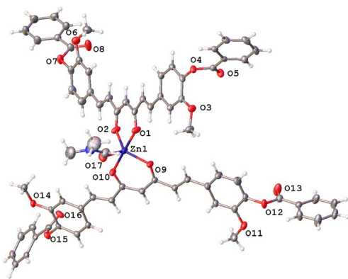
Fig. 5 Thermal ellipsoids of compound 8 , at 50% probability level.
