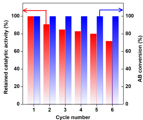
Fig. 7 Retained catalytic activity of the \text{Co}_{0.8}\text{Cu}_{0.2}\text{P}/\text{AC} and AB conversion in successive runs for AB hydrolysis.
