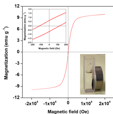
Fig. 6 Magnetic hysteresis loop of the prepared \text{Co}_{0.8}\text{Cu}_{0.2}\text{P/AC} (inset, optical photograph).
