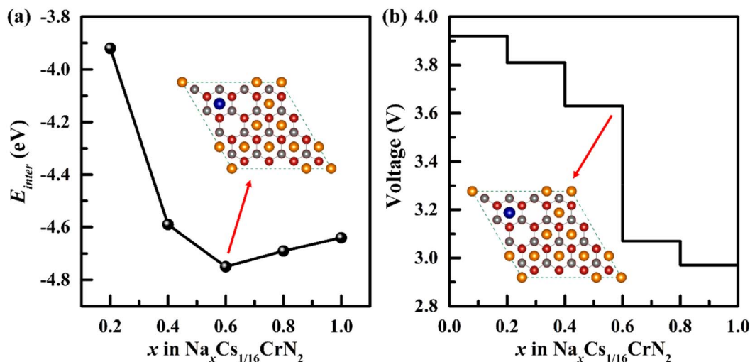
Fig. 5 (a) The intercalation energy ( E_{inter} ) of Na in Cs_{1/16}CrN_2 at various concentrations. (b) The voltage profile of Na embedded in Cs_{1/16}CrN_2 (the illustration shows the intercalation structure with a Na concentration of 0.6, and the most stable intercalation structure at each concentration is shown in Fig. S6†).
