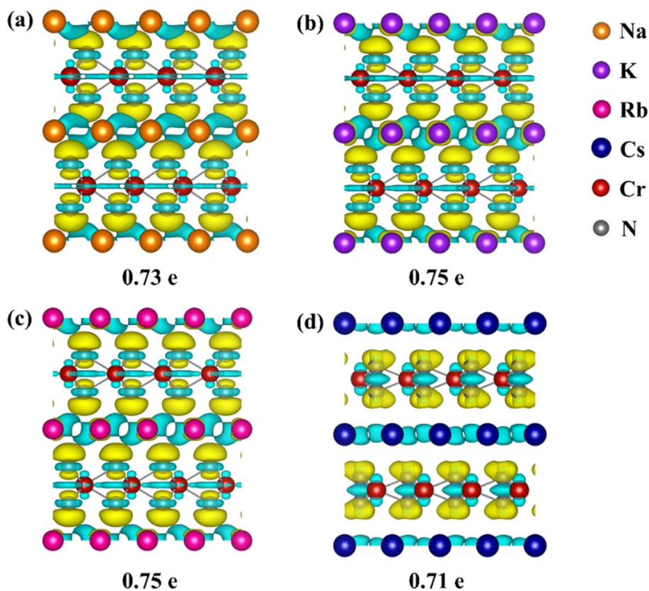
Fig. 6 Differential charge density and charge transfer for CrN_2 with Na (a) K (b) Rb (c) Cs (d) intercalation (orange, purple, rose, dark blue, dark red, and gray spheres represent Na, K, Rb, Cs, Cr, and N atoms, respectively. Yellow areas and light blue areas represent electron-rich regions and electron-deficient regions, respectively. The isosurface level is set to 0.003 e \text{ \AA}^{-3} ).
