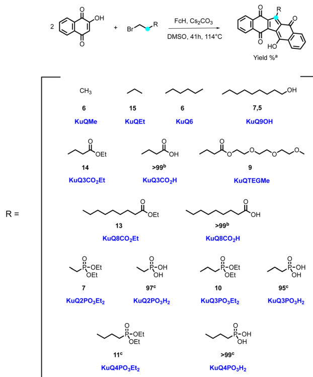
Scheme 1 One-pot synthesis of KuQ derivatives. Reaction conditions: 2-hydroxy-1,4-naphthoquinone 5.75 mmol, alkyl bromide 12 mmol, \text{Cs}_2\text{CO}_3 8 mmol, ferrocene (FcH) 0.033 mmol, DMSO 22 mL, 41 h, 114 °C. 23,25–27 (a) isolated yield; (b) quantitatively obtained through hydrolysis of the corresponding ester. Reaction conditions: 25 KuQXCO 2 Et (X = 3 or 8) 0.1 mmol in 8 mL THF, NaOH 25% in 2 mL MeOH, 1 h, rt. (c) Quantitatively obtained through hydrolysis of the corresponding phosphonate ester. Reaction conditions: 26 KuQXP(O) 3 -Et 2 (X = 2, 3 or 4) 0.1 mmol, NaI 5 mmol, bromotrimethylsilane 5 mmol, 16 mL dry CH 3 CN:CHCl 3 , 4 h, 40 °C, N 2 atmosphere. Then 30 mL MeOH, 1 h, rt.
