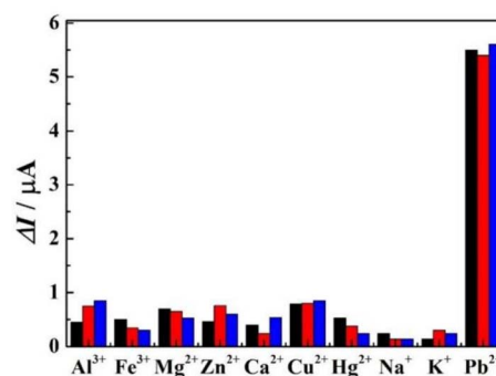
Fig. 6 The specificity of r-PHIS/GO/GCE for \text{Pb}^{2+} detection.
