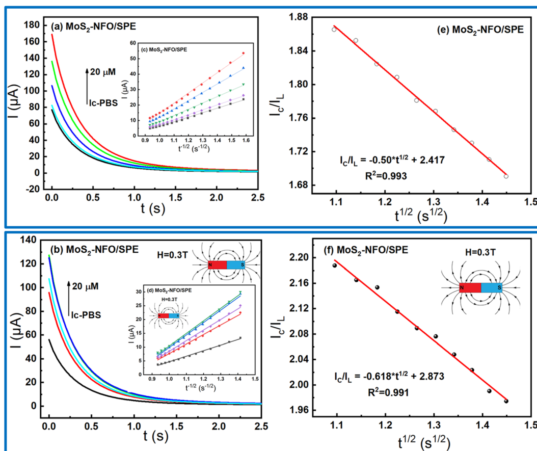
Fig. 6 (a and b) Chronoamperograms obtained at \text{MoS}_2 -NFO in 0.1 M PBS containing various concentrations of CLB with and without external MF; (c and d) plots of I vs. t^{-1/2} ; (e and f) plots of I_c/I_L vs. t^{1/2} at 15 \mu\text{M} CLB in 0.1 M PBS buffer.
