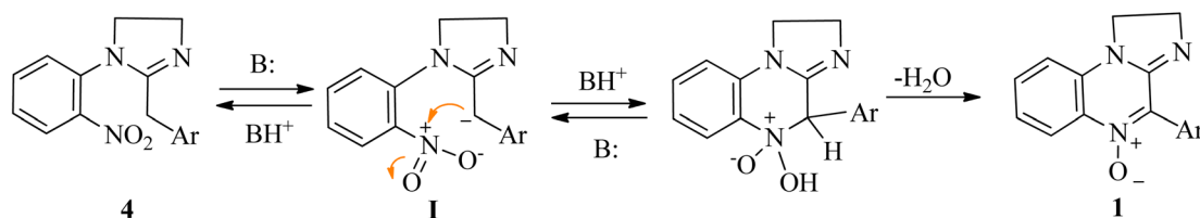
Scheme 3 Probable base-promoted cyclodehydration mechanism.
