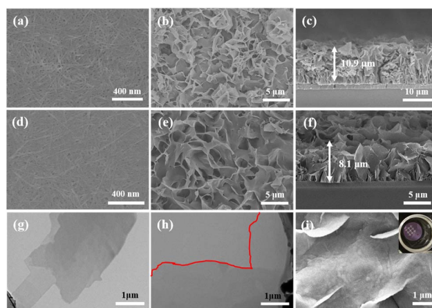
Fig. 1 (a) SEM surface and corresponding cross-sectional images of (a) pristine CuHNs; (b) and (c) pristine Cu-TCPP membrane "C _{0-0} "; (d) PSS-SSP@CuHNs, (e) and (f) PSS-SSP@Cu-TCPP membrane "C _{1-1} "; TEM images of (g) C _{0-0} ; (h) C _{1-1} and (i) SEM surface image of C _{1-1} membrane with deposited Ag electrodes (the picture of C _{1-1} membrane with attached Ag electrodes).
