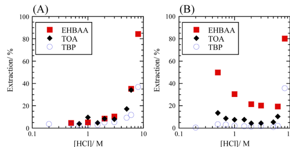
Fig. 2 Extraction percentage of Se as a function of HCl concentration. (A) SolAxH: Se IV O 2 dissolved and (B) SolBxH: Na 2 Se VI O 4 ·10H 2 O dissolved. Organic phase, 0.5 M EHBA, TOA, or TBP pre-equilibrated with HCl; aqueous phase, [Se] = 0.001 M.
