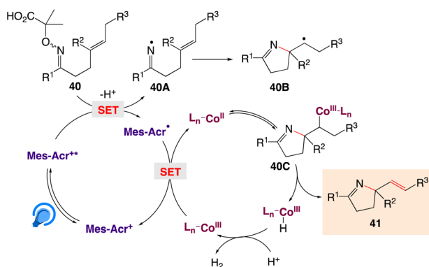
Scheme 27 Proposed Mechanism for synthesis of alkene-containing N -heterocycles.
