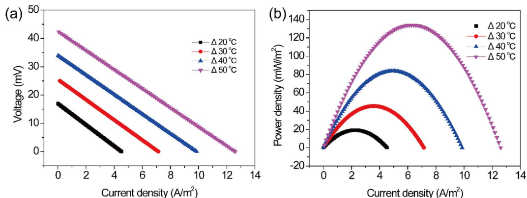
Fig. 6 (a) Polarization and (b) power density curves at different temperature differences.
