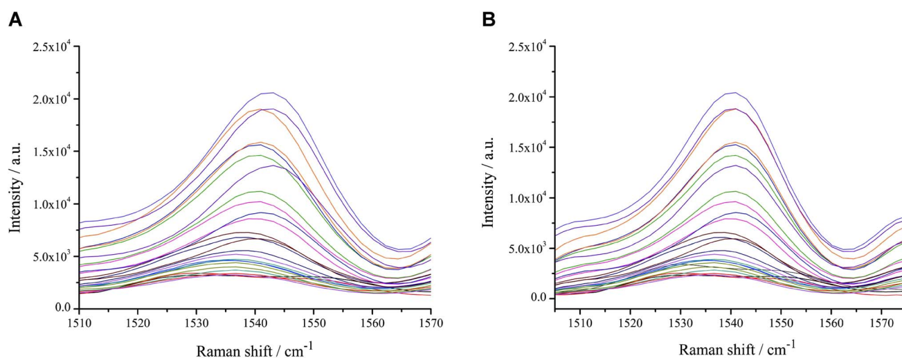
Fig. 5 Illustration of band alignment of the spectra of the DPD-basic orange 21 mixtures before (A) and after (B) spectra calibration, concerning the 1536 cm -1 band.
